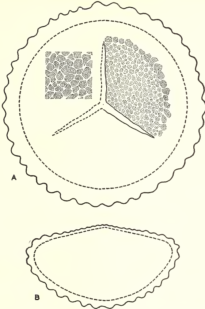
TEXT-FIG. 2. Verrucosisporites contactus sp. nov. Diagrammatic reconstructions. A, Polar aspect, proximal on the right-hand side showing the differentiated contact areas and the form of the distal verrucae bases on the left-hand side. B, Polar section. \times 1,000 .
